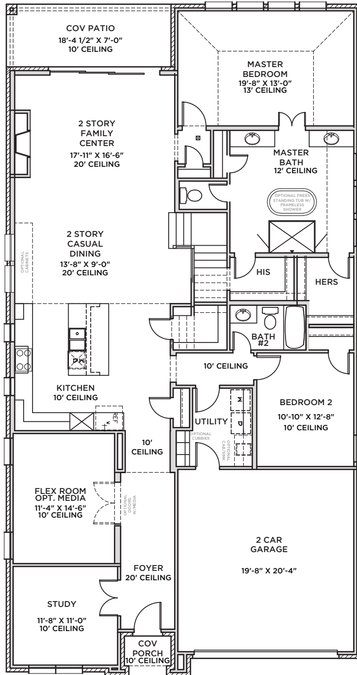
FIRST FLOOR
