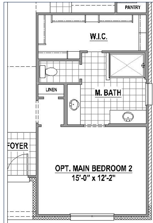
1st Floor Main Bedroom ILO Bedroom 2
