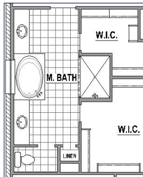
Drop-in Tub at Main Bath
