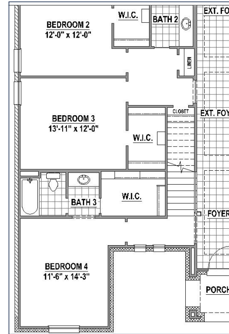
Stair Location w/ 2nd Floor Options
