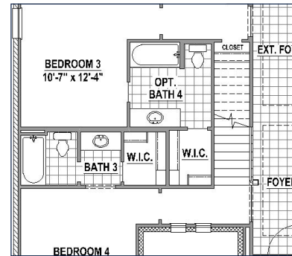
Bath 4 w/ Stairs to 2nd Floor Options
