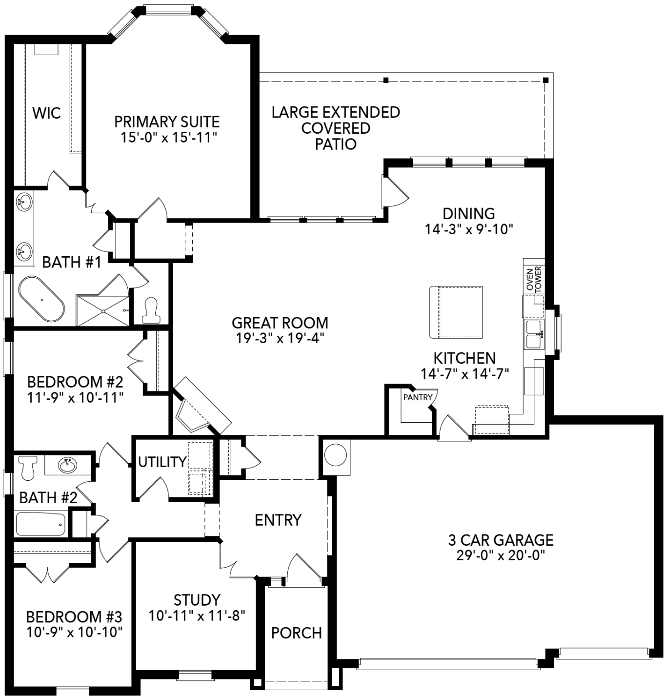
First Floor
