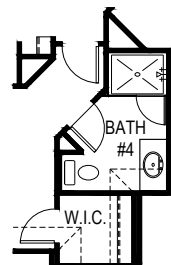
OPTIONAL BATH #4 W/ ELEV'S: E & Q
