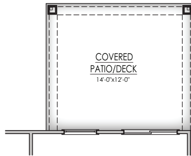
1 - OPT COVERED PORCH
