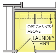
6 - OPT CABS. @ LAUNDRY
