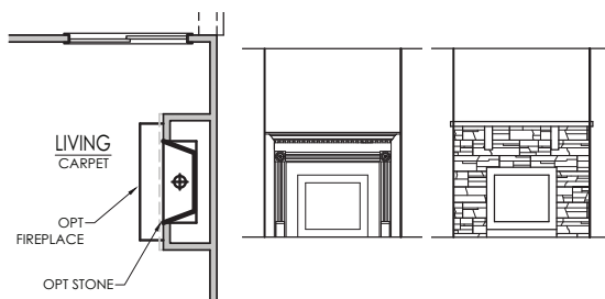
4 - OPT GAS FIREPLACE
