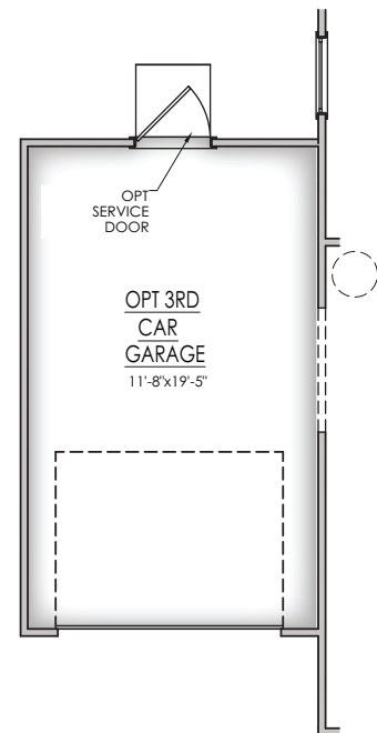
10 - OPT SERVICE DOOR @ 3RD CAR GARAGE
