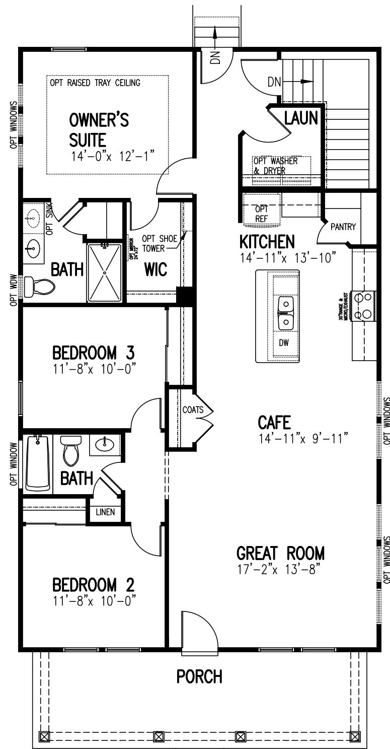
1st Floor Plan Based on Elevation L
