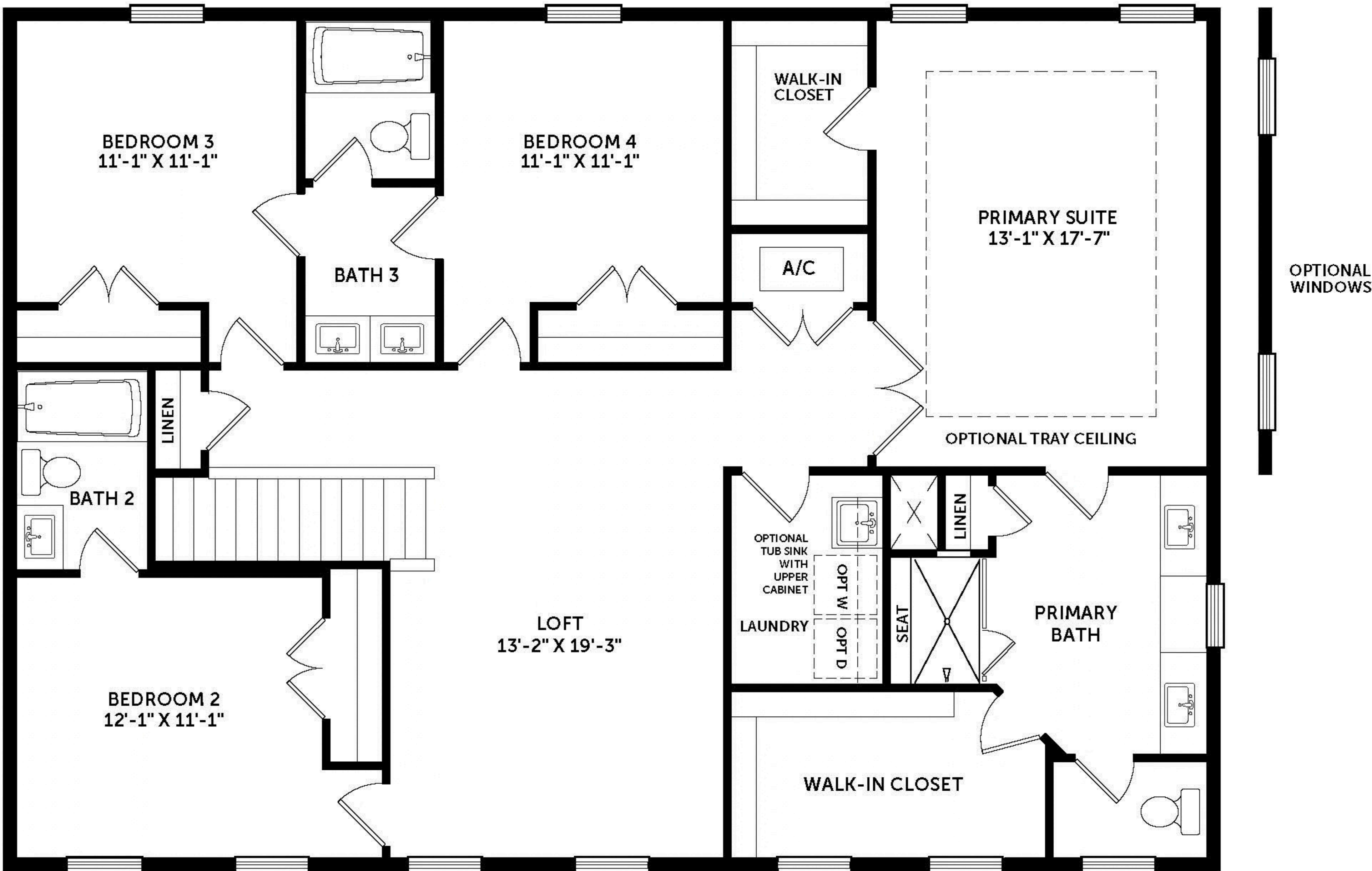
SECOND FLOOR 8' CEILING
