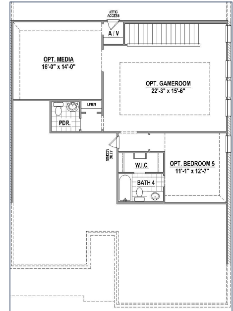
Game Room, Media Room, Bedroom 5 w/ Bath 4 and Powder Bath (+979 SF)
