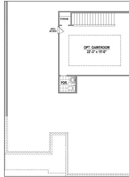
Game Room (+448 SF)
