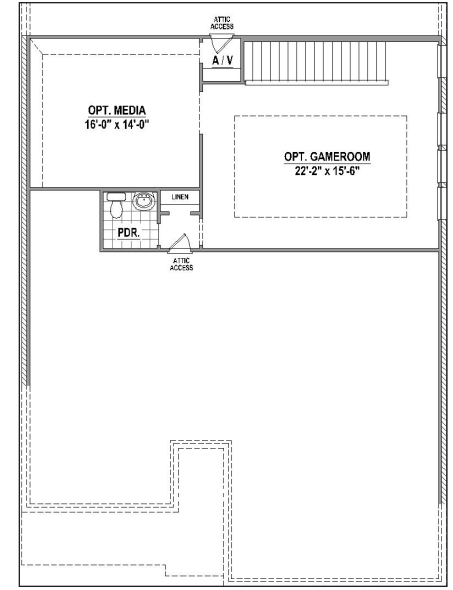
Game Room & Media Room w/ Powder Bath (+714 SF)
