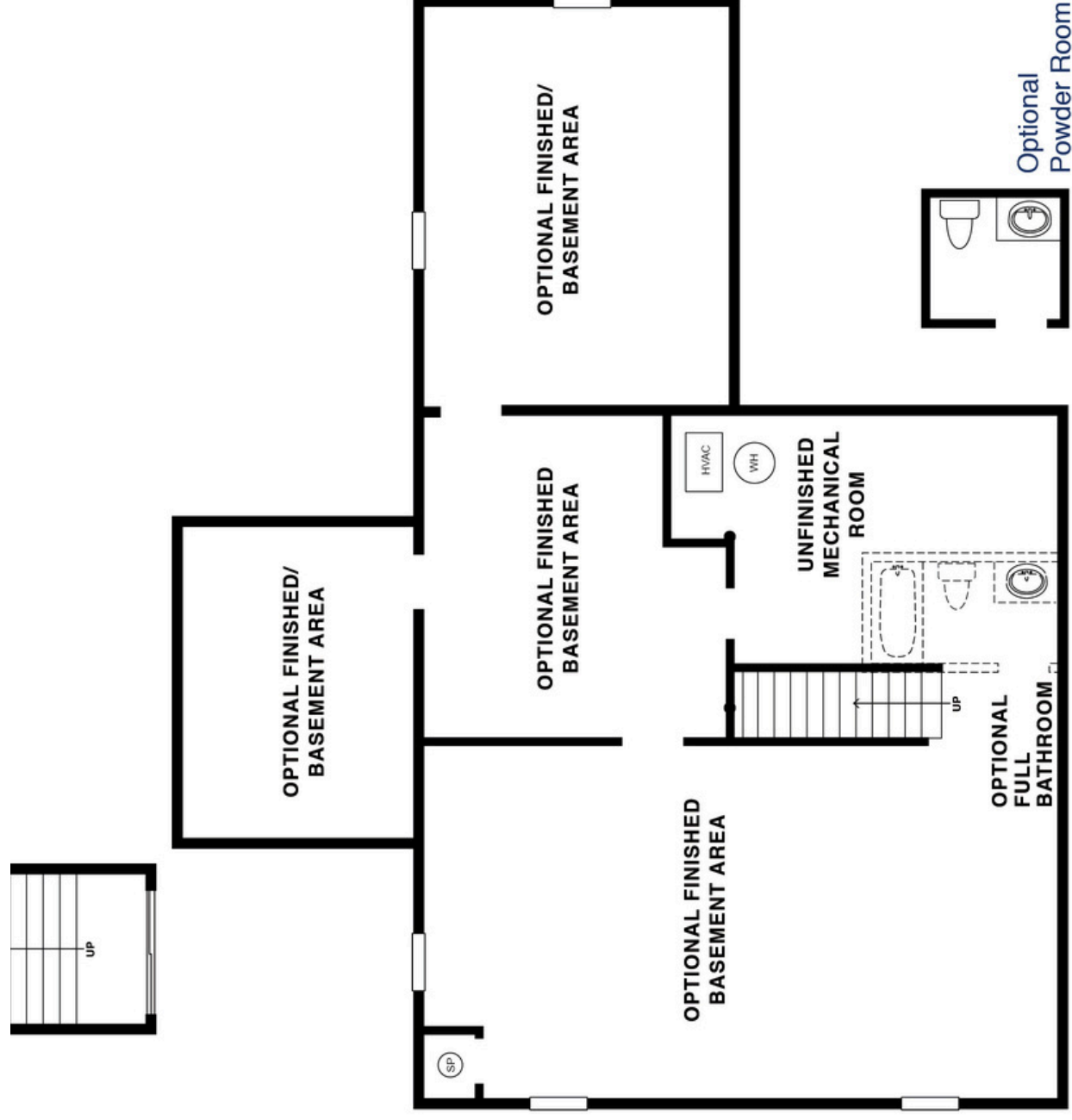
Basement
