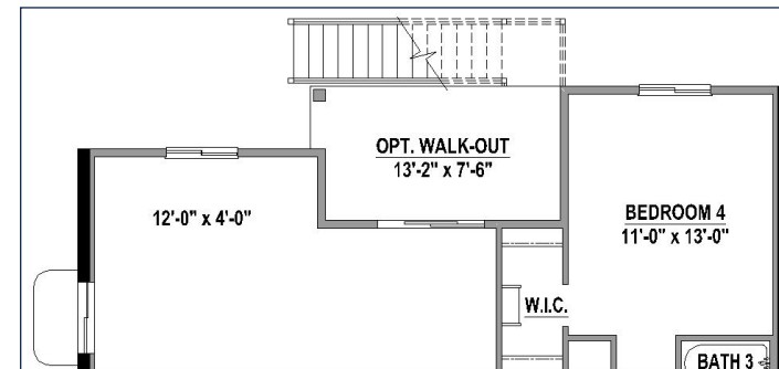
Optional Walkout Basement with Deck Above
