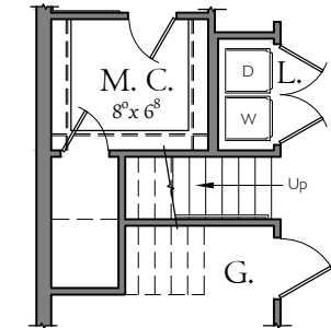
STAIRS LAYOUT
