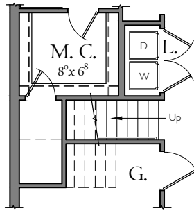
STAIRS LAYOUT
