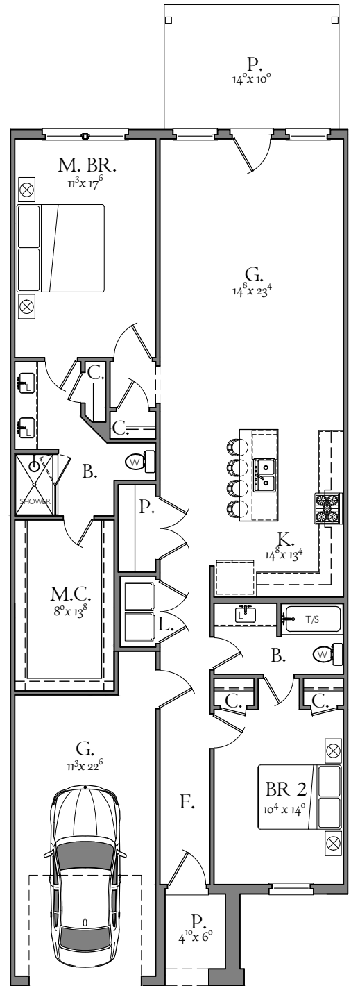
MAIN LEVEL -Single Garage
