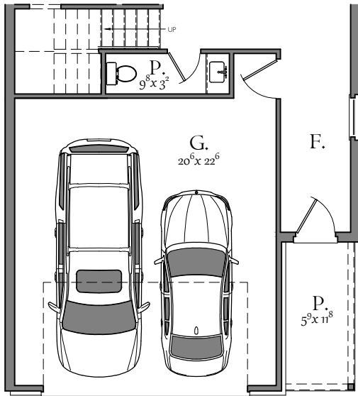
MAIN LEVEL -Double Garage
