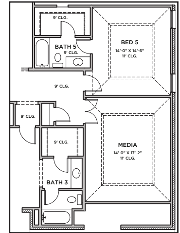
OPT MEDIA W/ OPT BED 5 & BATH 5
