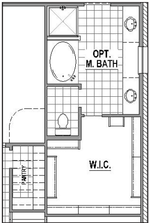
Alternate Main Bath Layout
