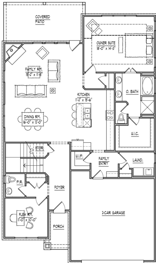
FIRST FLOOR PLAN ELEVATION A
