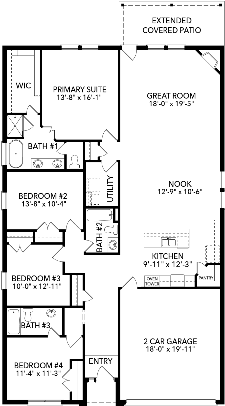
First Floor
