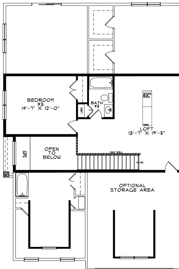
SECOND FLOOR
