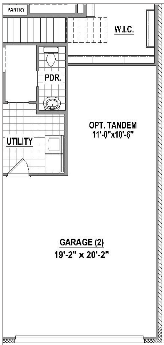
Optional Tandem Garage with 2nd Floor (-161 SF)
