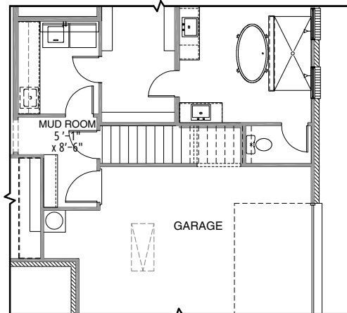
STAIRS W/ OPT. 2ND FLOOR
