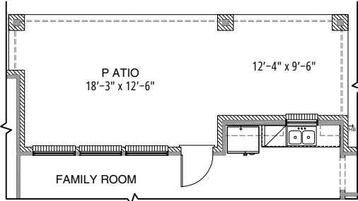
OPT. EXPANDED PATIO
