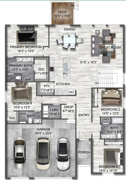
MAIN LEVEL
