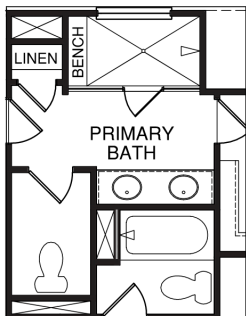
ENLARGED SHOWER
