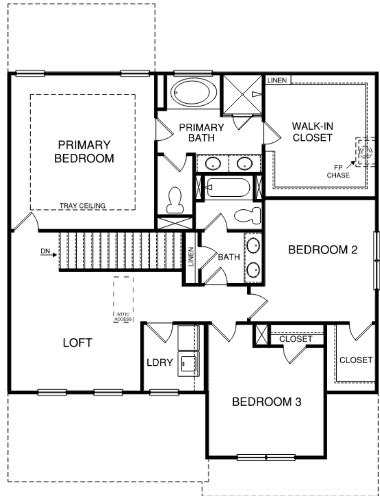
SECOND FLOOR
