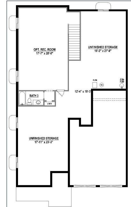
Optional Rec Room w/Bath 3 (+734 SF)
