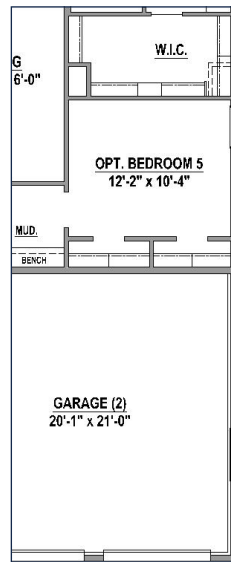
Optional Bed 5 **Option not available w/Opt. Alt Main Bath Layout
