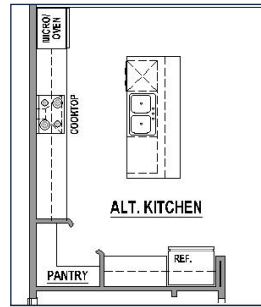
Optional Alternate Kitchen Layout
