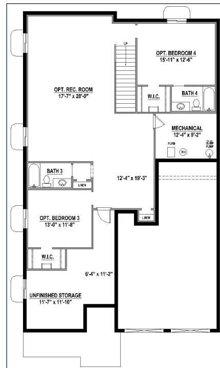
Optional Rec Room, Beds 3 & 4 w/Baths 3 & 4 (+1,499 SF)
