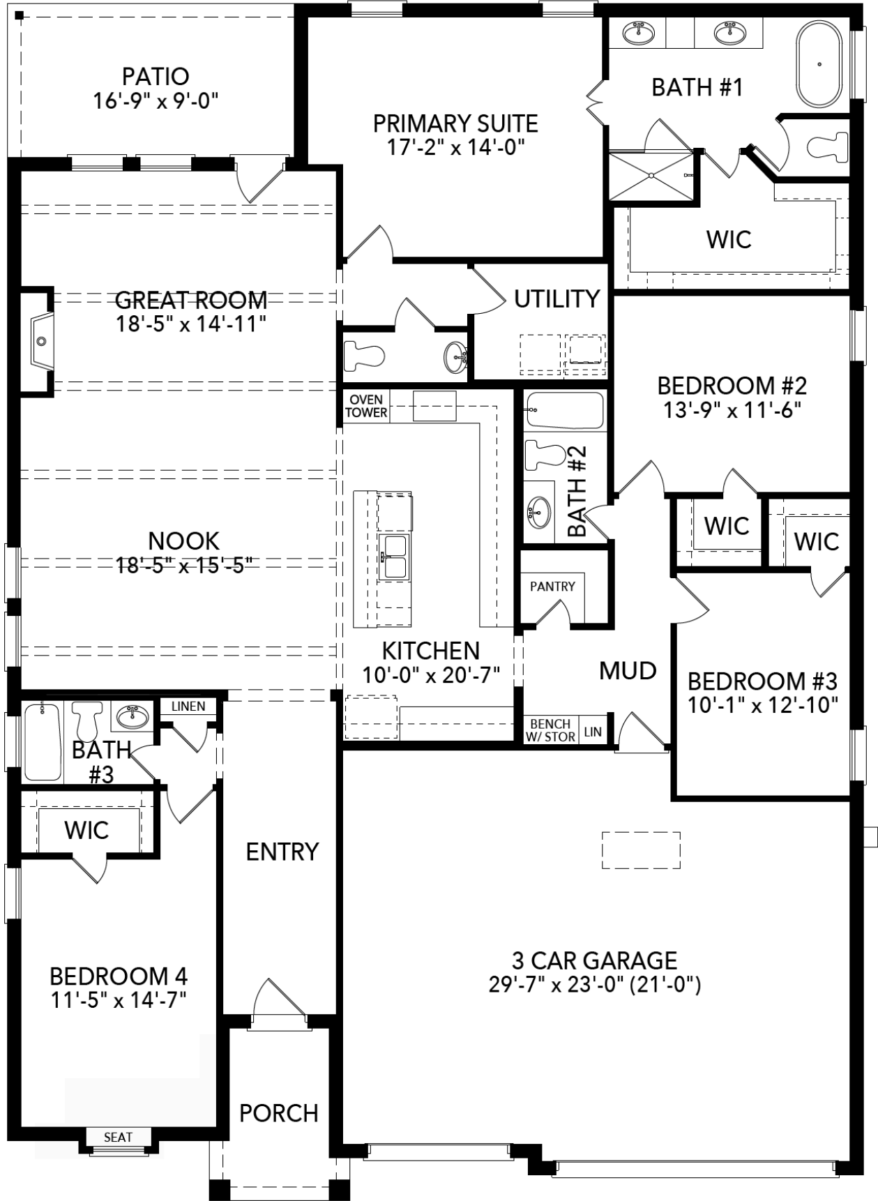
First Floor
