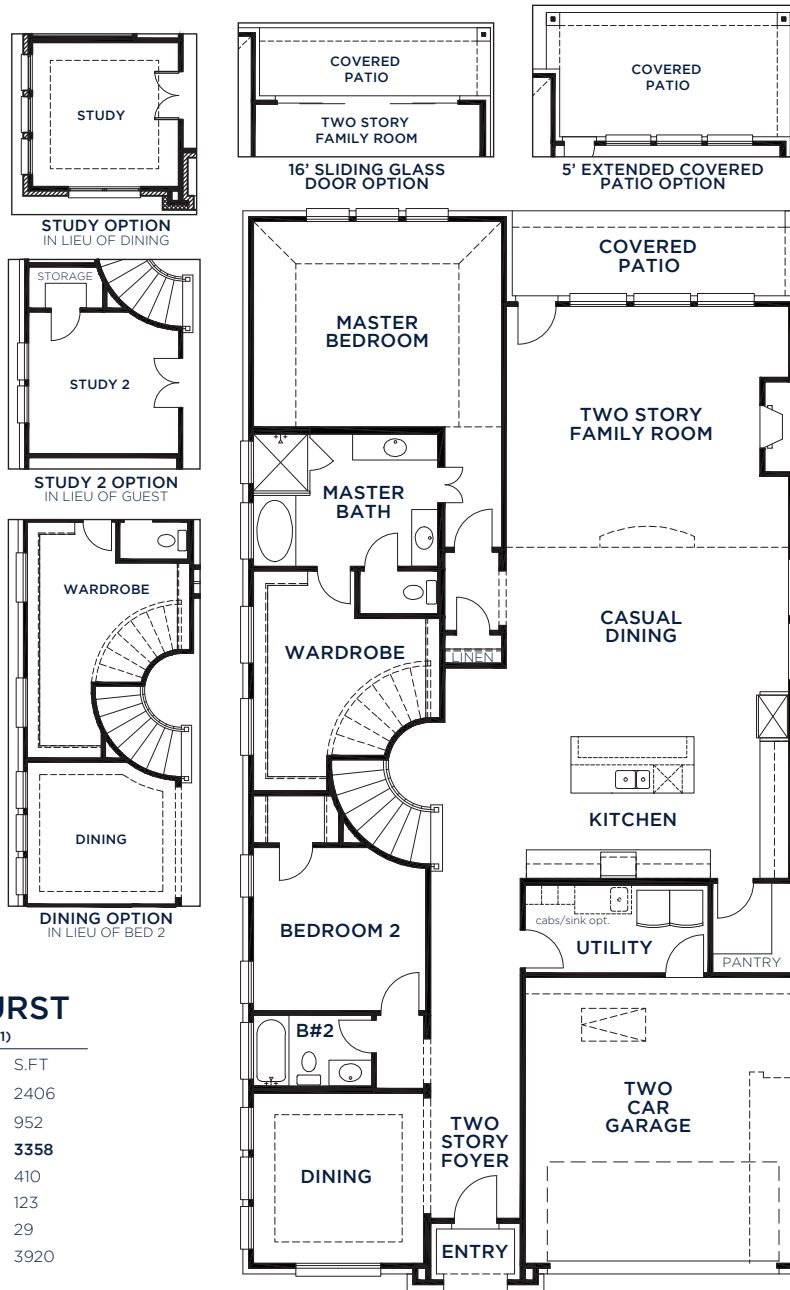
FIRST FLOOR
