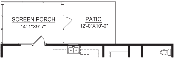
OPT. SCREEN PORCH
