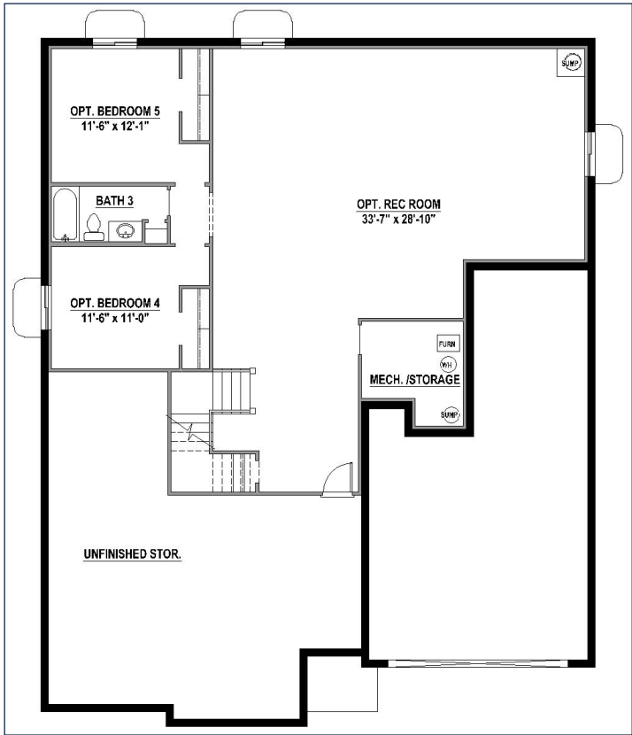
Rec Room, Bedrooms 4 & 5 w/ Bath 3 (+1,653 SF)
