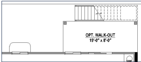
Basement Walkout w/ Deck Above
