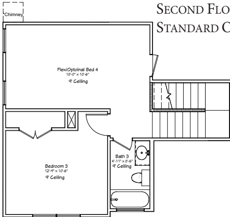
SECOND FLOOR 4TH BEDROOM OPTION:
