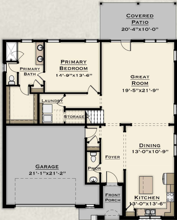
Main Level C
