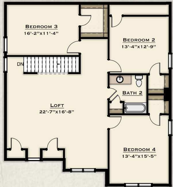
Second Floor B
