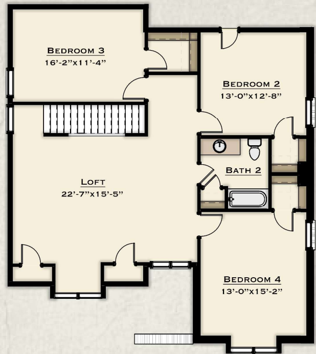
Second Floor C
