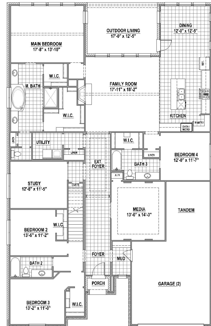
Alternate First Floor Layout with Optional Second Floor
