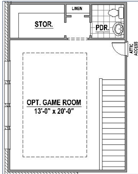
Optional Game Room with Powder Bath & Storage (+439 SF)
