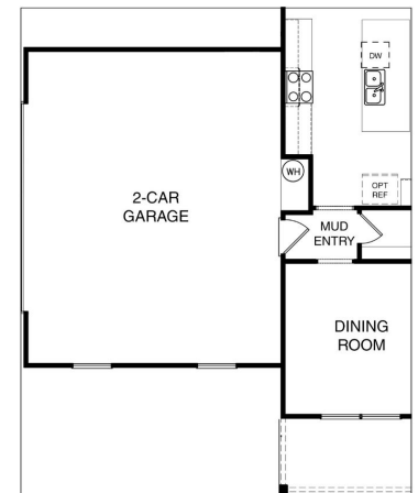
2-CAR SIDE ENTRY GARAGE
