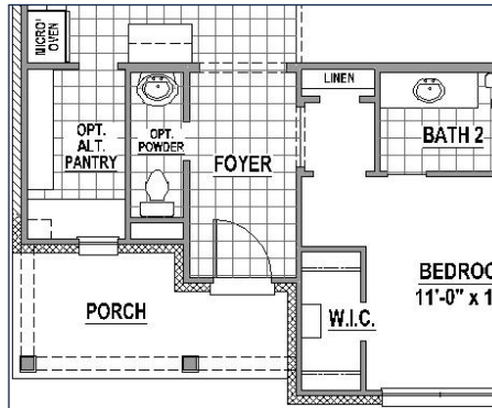
Alternate Pantry Layout w/ Powder Bath
