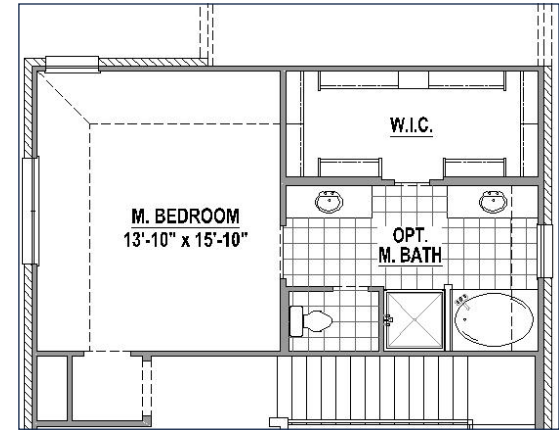
Alternate Main Bath Layout
