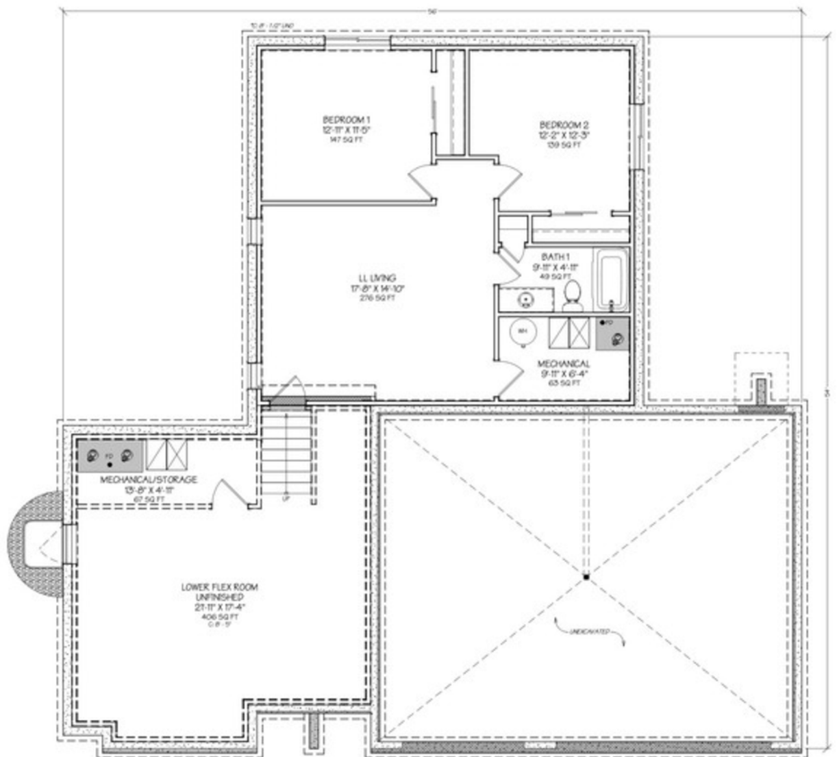
Mia 3.0 - Base Plan - Lower Floor - 850 sq ft
