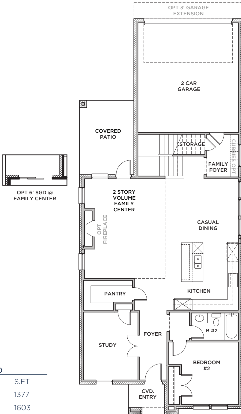
FIRST FLOOR
