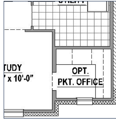
Pocket Office ILO Storage at Study
