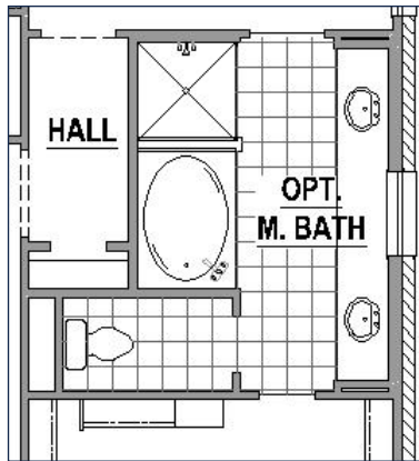
Alternate Main Bath Layout
