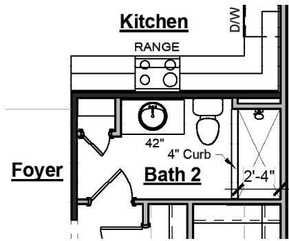
Bath 2 Tile Shower
