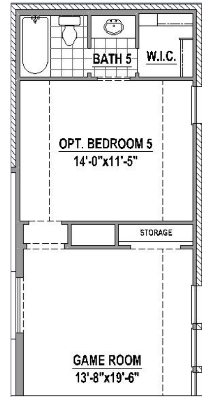
Bedroom 5 w/ Bath 5 (+301 SF)
