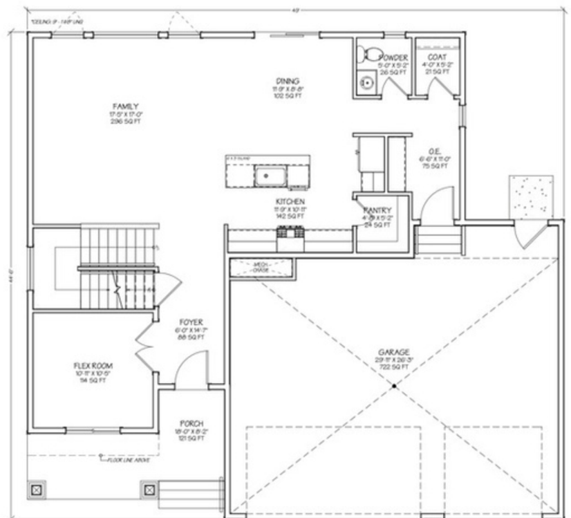
Augusta 3.0 - Base Plan - Main Floor - 1,078 sq ft
