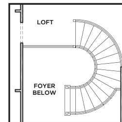
UPPER LEVEL OPT CURVED STAIR
