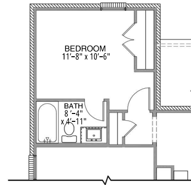
OPT. ADDITIONAL BEDROOM/ BATH
