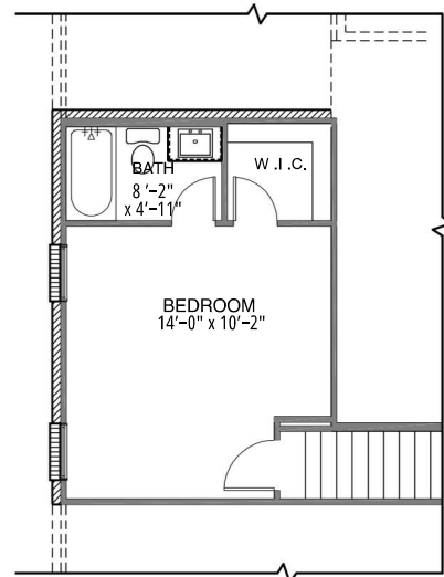
OPT. ADDITIONAL UPSTAIRS BEDROOM/ BATH
