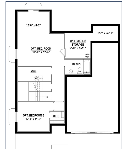
Optional Rec Room, Bed 6 w/Bath 3 (+843 SF)
