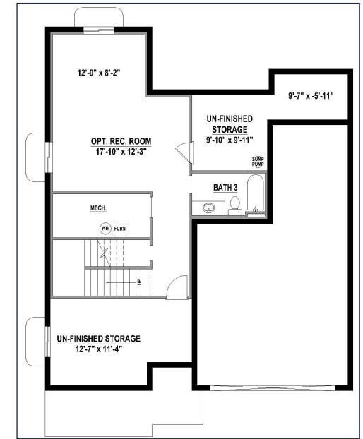
Optional Rec Room with Bath 3 (+632 SF)
