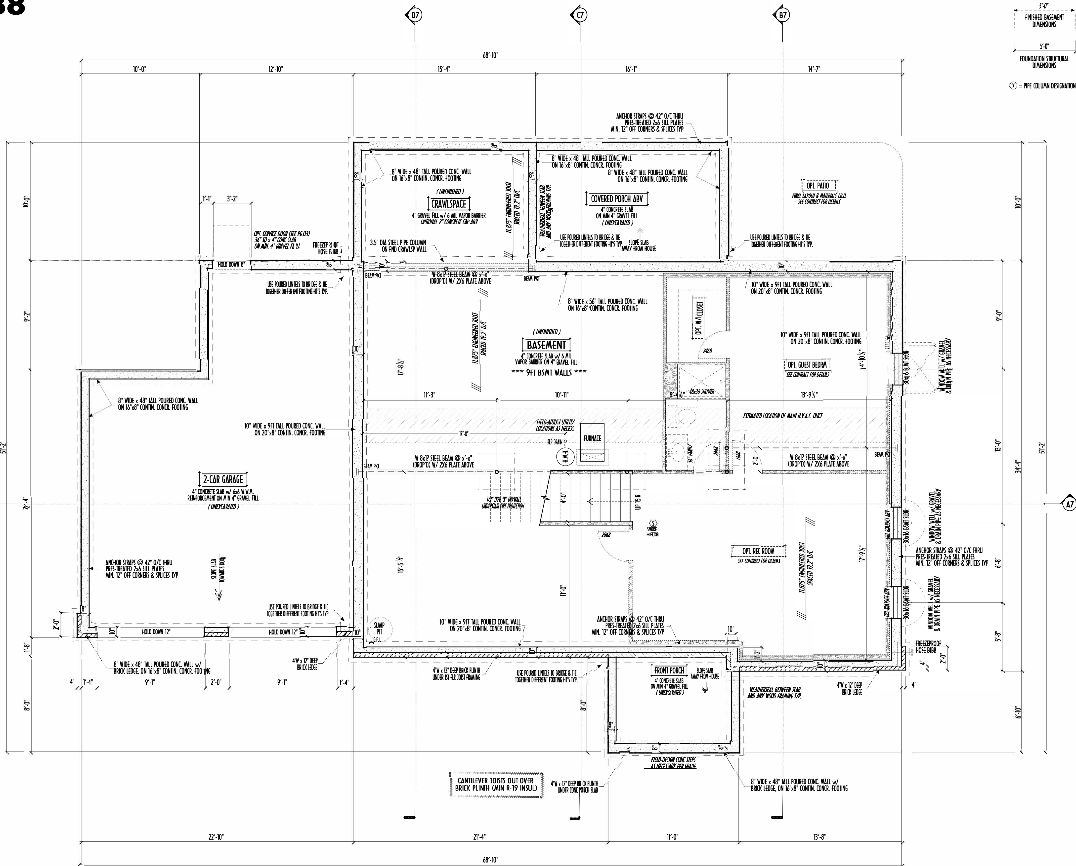
FOUNDATION / BASEMENT PLAN SCALE: 1/4" = 1'-0"
