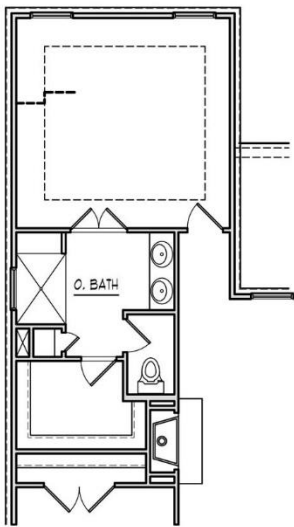
OPTIONAL OWNER BATH W/ SUPER SHOWER
