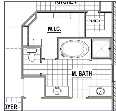
Drop In Tub at Alternate Main Bath
