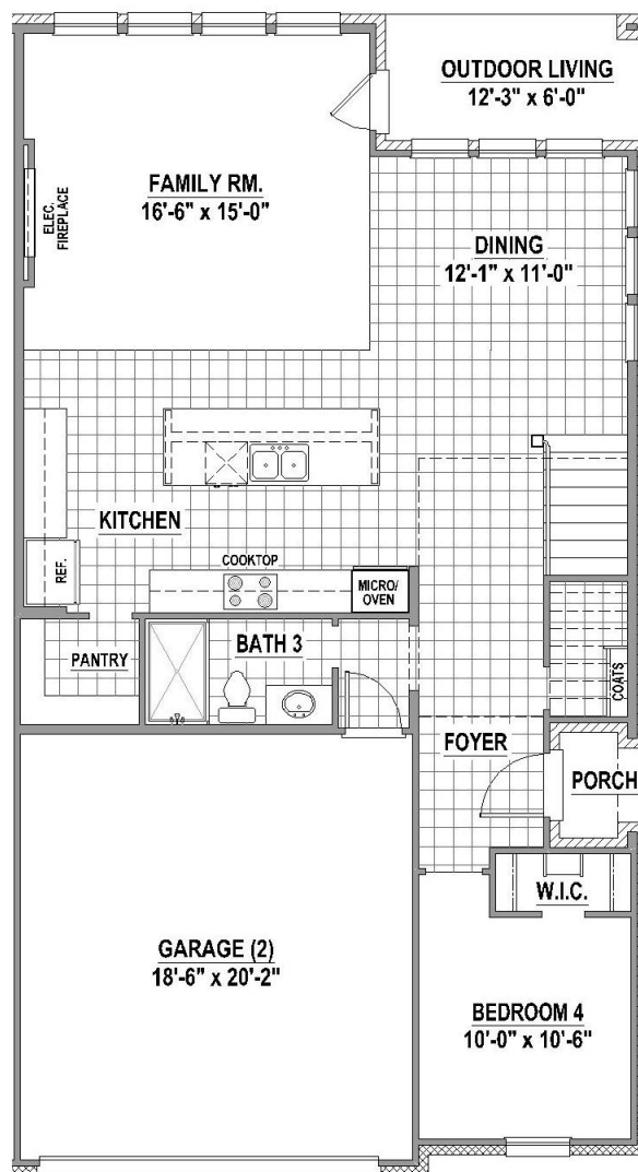
1 st Floor
