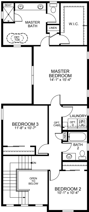
SECOND FLOOR
