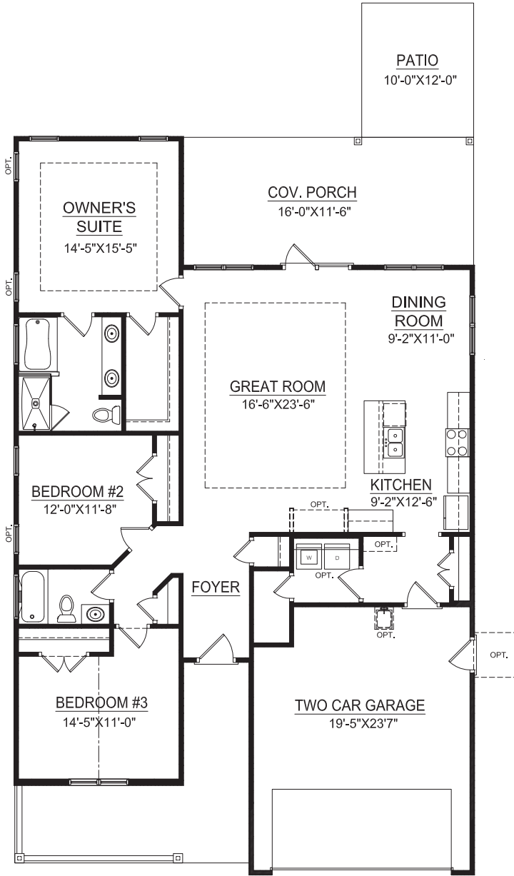
FLOOR PLAN
