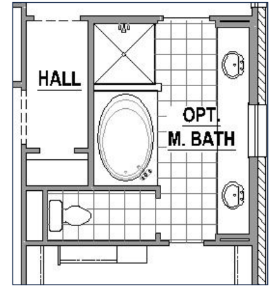
Alternate Main Bath Layout w/ Drop-In Tub
