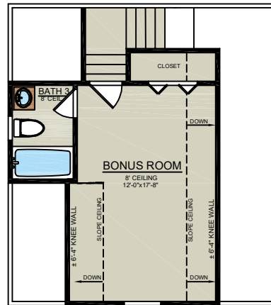
BONUS ROOM w/BATH OPTION BONUS ROOM w/BATH 347 SF
