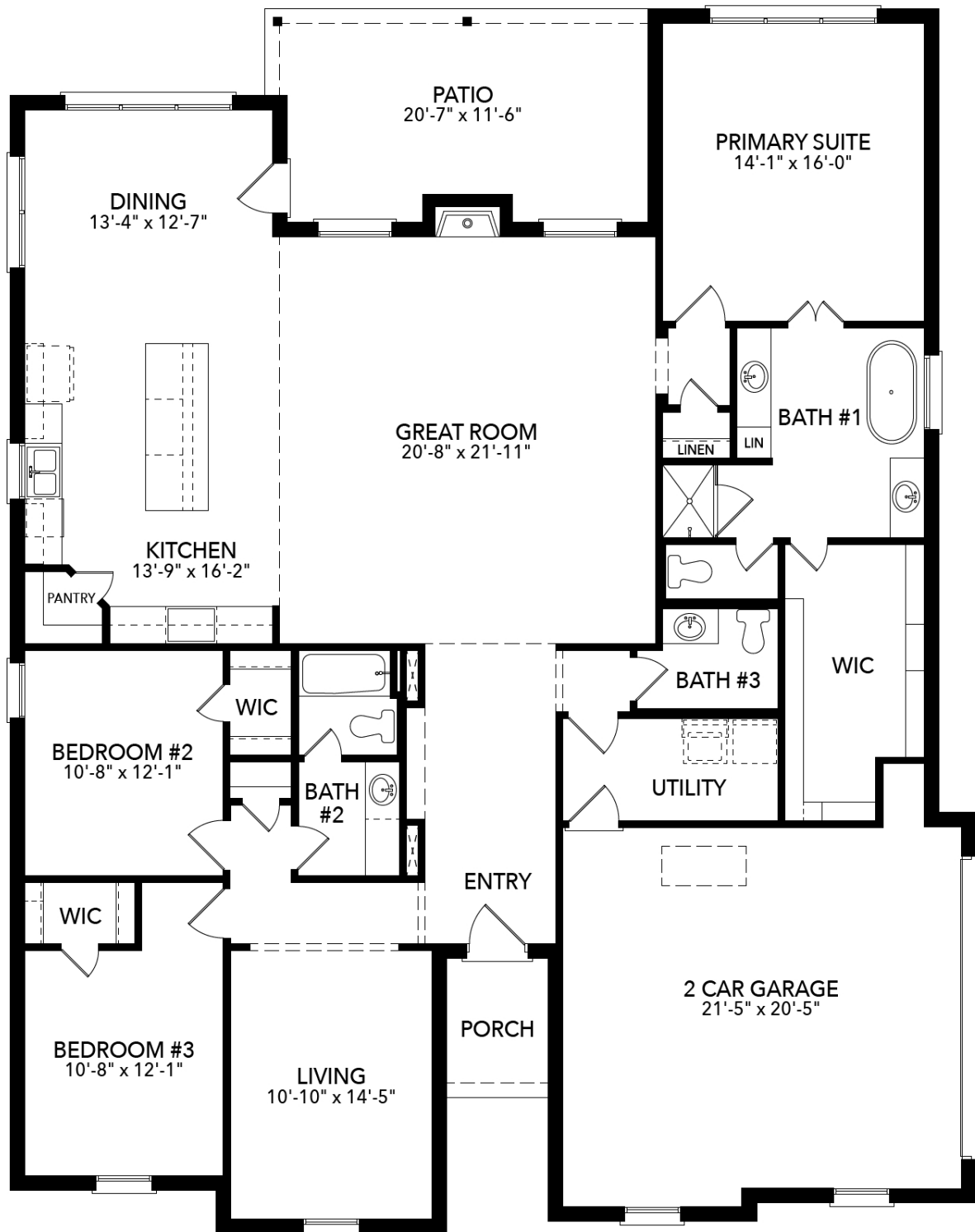
First Floor
