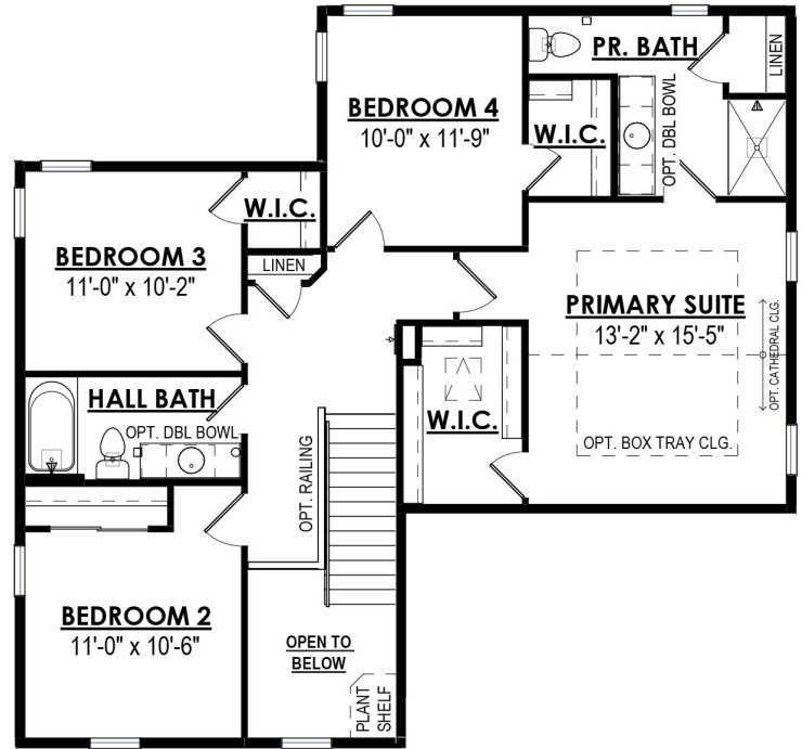
2nd FLOOR 1,087 Sq. Ft.
